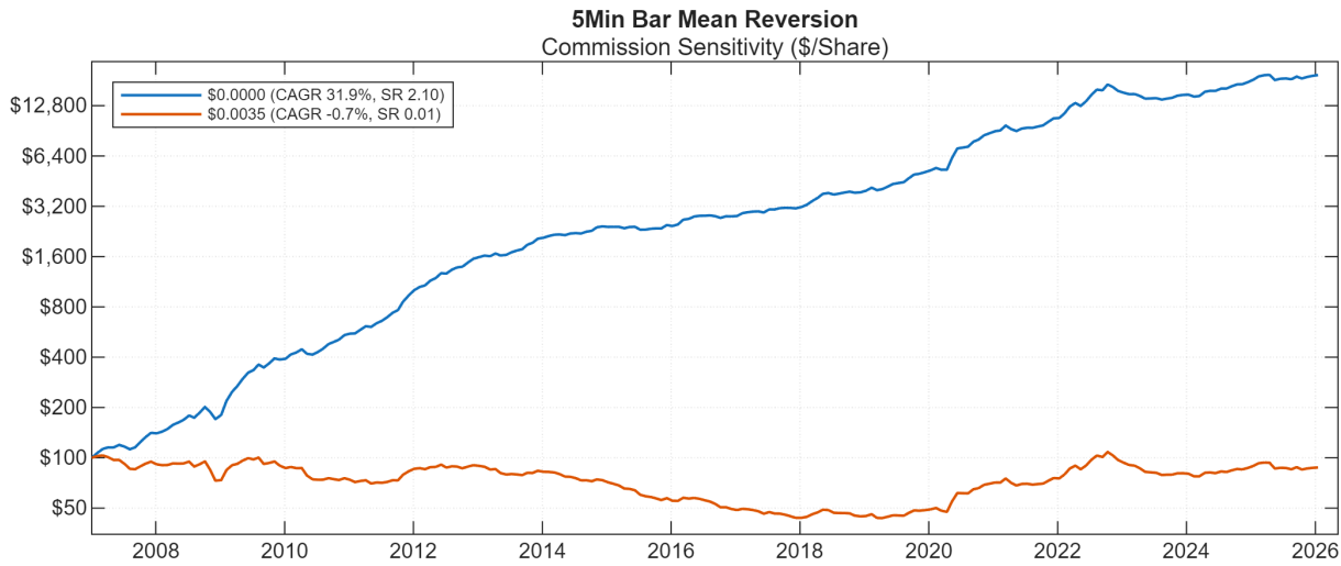
Figure 2: Sensitivity of the fast alpha signal ( N = 1 ) to IBKR standard-tier commission rate. The signal uses the sign of the most recent bar's return as a mean-reversion cue, taking the opposite position on the following 5-minute bar. Despite strong gross-of-fee performance, transaction costs completely erode its profitability.
