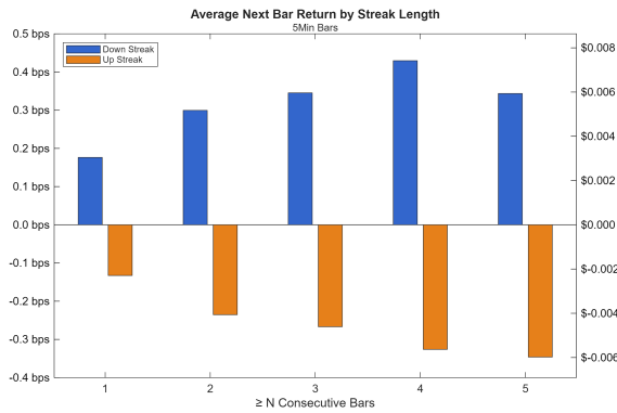
Figure 1: Average return (in bps and $/share) of bar t+1 following a streak of at least N consecutive bars in the same direction, illustrating the presence of a mean-reversion effect.
